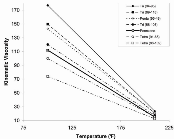
Figure 4 – Kinematic viscosity as a function of temperature for a series of silahydrocarbons [48]
