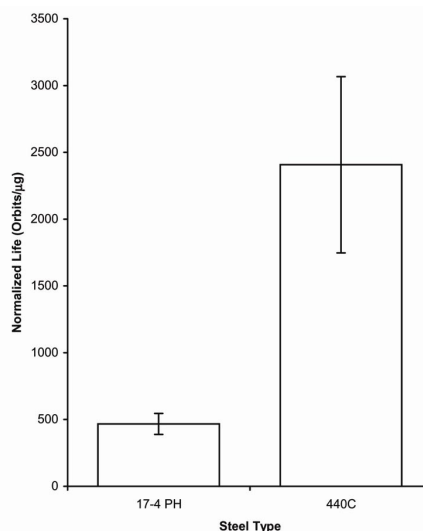
Figure 15 – Relative life of Pennzane® SHF-X2000 on two different bearing steels
