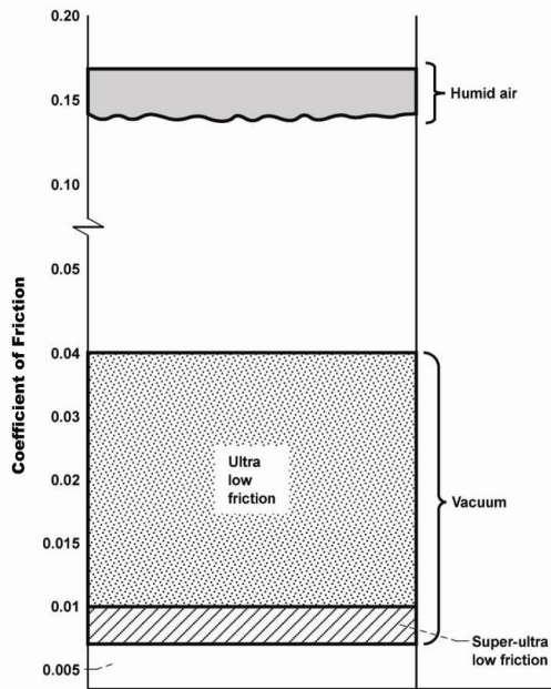
Figure 14 – Friction variation of sputtered MoS 2 films [95]
