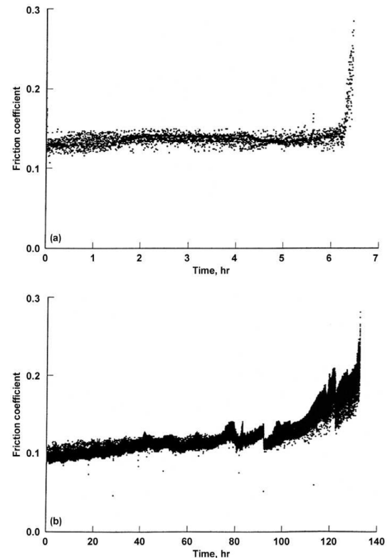
Figure 11 – Coefficient of friction as a function of time for (a) Krytox ™ 143AC and (b) Pennzane ® SHF-X2000 (spiral orbit rolling contact tribometer – note time scale difference)
